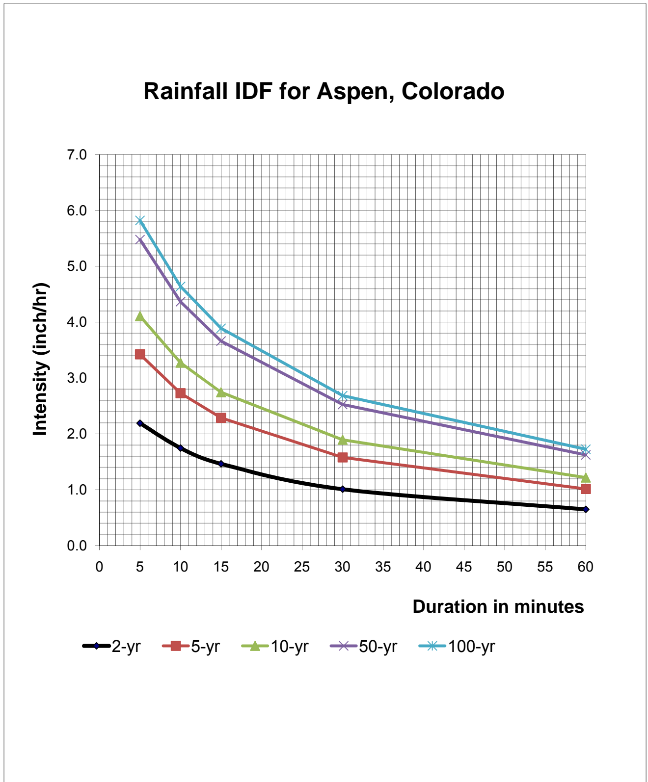
Figure 2.1 IDF Curves for Aspen, Colorado
